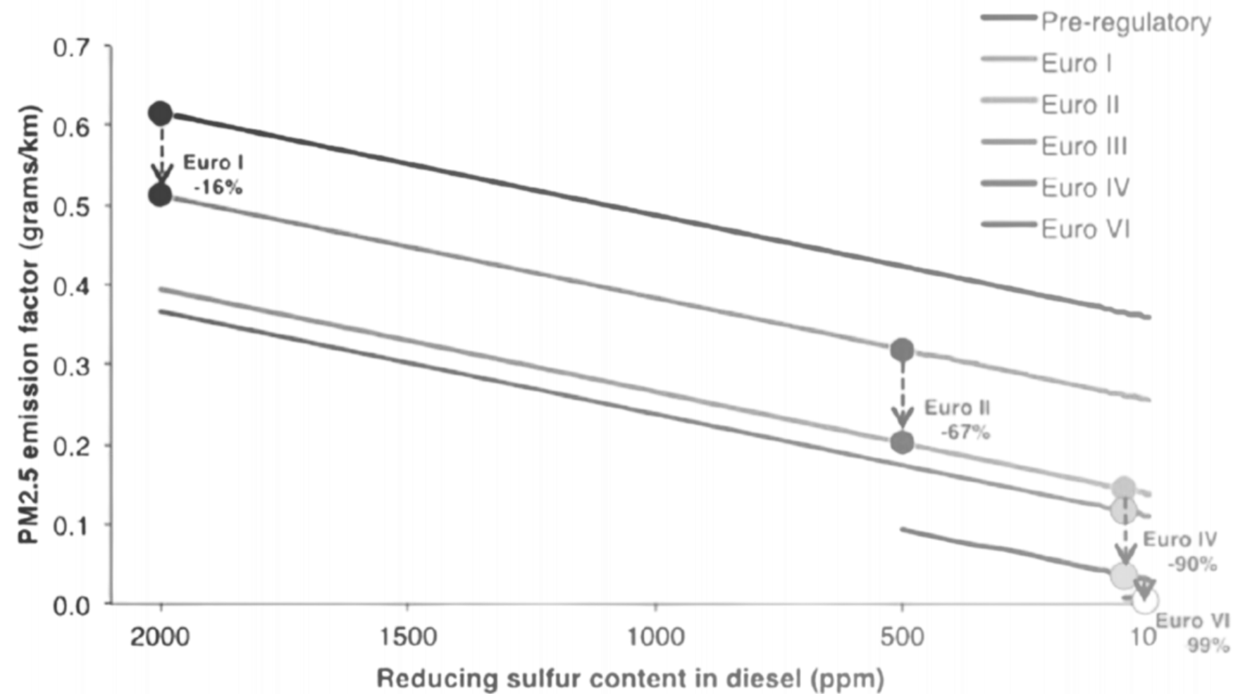
Figure 1.2. Impact of fuel sulfur levels and emissions control standards on PM 2.5 emissions from heavy-duty diesel vehicles (grams/km)
